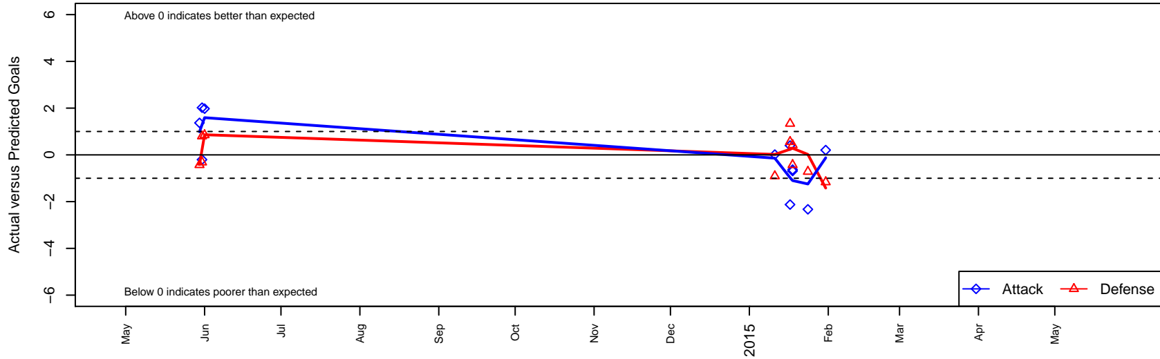
Academy Idaho Cads B96 Dots are actual minus expected GF (blue circles) and GA (red triangles). Blue line is smoothed change in attack strength. Red is smoothed change in defense strength.
